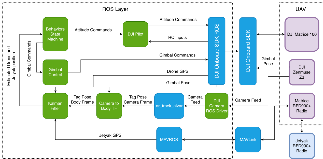
FIGURE 3 Block diagram of the developed UAV system architecture. The blue blocks are open-source ROS layers, the green blocks are components developed for this project, the magenta blocks are the hardware peripherals of the UAV, and the cyan one is hardware peripherals of the ASV. ASV, Autonomous Surface Vehicle; ROS, Robot Operating System; UAV, Unmanned Aerial Vehicle [Color figure can be viewed at wileyonlinelibrary.com ]
