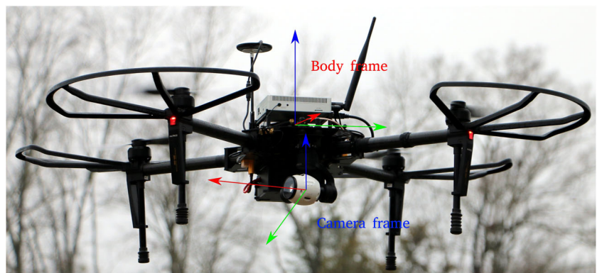
FIGURE 4 The body and camera coordinate systems shown on the UAV. Since the camera is mounted on a gimbal it is free to rotate relative to the body. UAV, Unmanned Aerial Vehicle [Color figure can be viewed at wileyonlinelibrary.com ]
