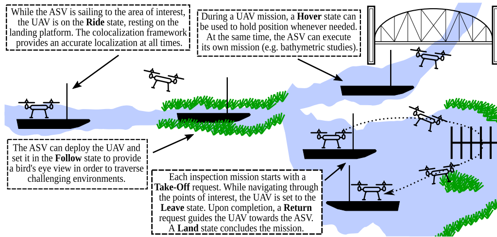
FIGURE 8 Concept design highlighting the characteristics of the UAV-USV marsupial system. For each phase of the sample mission the relevant high-level behavior state is provided. ASV, Autonomous Surface Vehicle; UAV, Unmanned Aerial Vehicle; USV, Unmanned Surface Vehicle [Color figure can be viewed at wileyonlinelibrary.com ]
