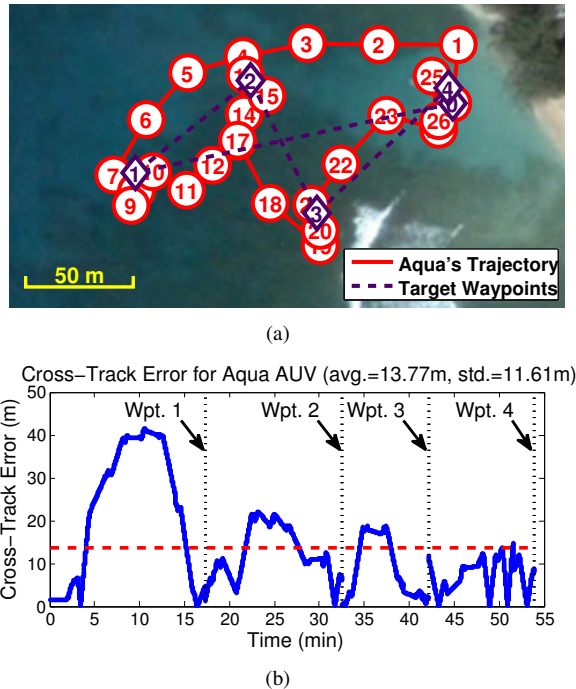
Fig. 10. (a) Overhead view of the Aqua AUV's trajectory. Diamond icons depict target locations suggested by the biologist for further inspection. Circular icons denote porpoising ascents during this session. (b) The cross-track error for Aqua's trajectory suggests that it was pushed off-course due to strong currents.
