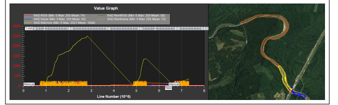
Fig. 9. Analysis of 3 ASVs at the Congaree river with two BSs. Map on the right shows three paths of ASVs. Path colors correspond to quality of communication: Blue-receiving error of less than 20%, yellow-up to 49%, orange- above 50% which considered unreliable for monitoring.
