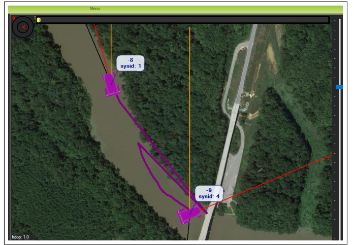
Fig. 3. Live monitoring of 2 ASVs communicating with 1 GCS at the Congaree river in South Carolina using Mission Planner (Ground Control Software).
