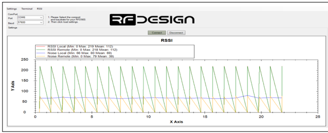
Fig. 10. Initial plot of RSSI and Noise values (Y-Axis) over Time (X-Axis) when a third node (BS or ASV) was added. We can observe the impact of introducing a new node on the quality of communication (RSSI and noise).
