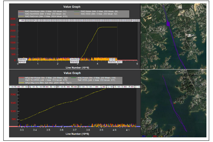
Fig. 8. Analysis example of local and remote RSSI (blue and orange), noise (red and green), and receiving error (yellow) values over distance of a remote (ASV) and a local node (BS) deployed at Lake Murray in LOS. Top map shows the full path and corresponding analysis on the left side of the map. Bottom shows a zoomed in view (segment of path and plot) when accumulated receiving error go beyond 20%.
