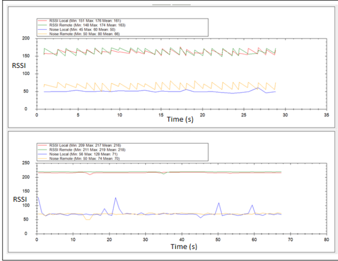
Fig. 11. Plot showing optimal RSSI Vs. Noise values (Y-Axis) over Time (X-Axis) of local and remote nodes (BS and ASV respectively) when communicating in point-to-point (bottom) and multi-point (top) scenarios
