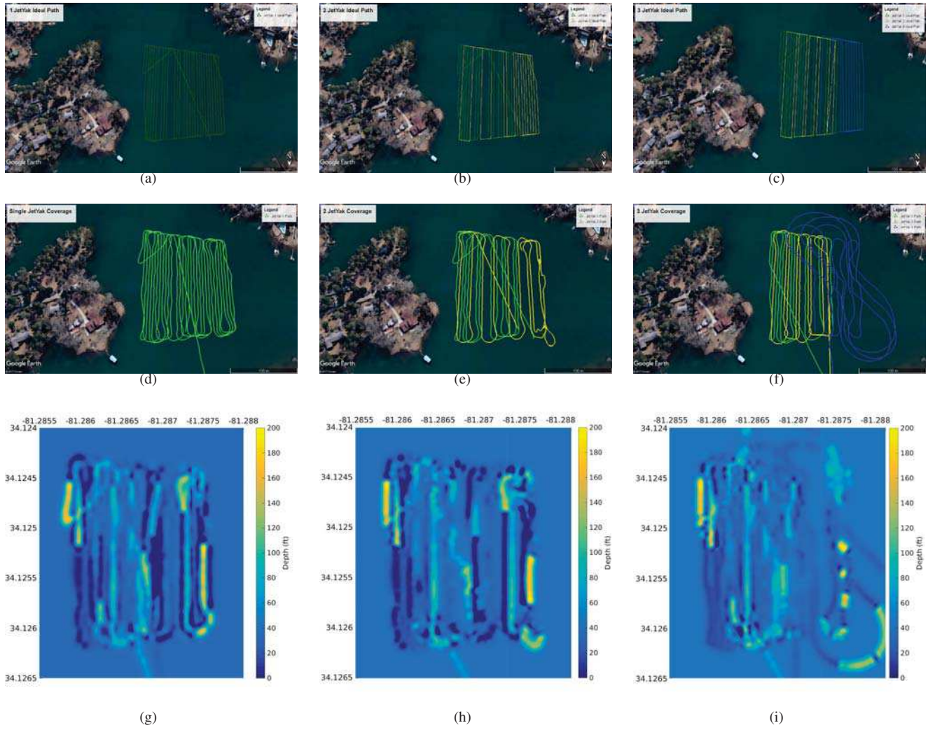
Fig. 5. Multi-robot experiments at Lake Murray, SC, USA. (b) Ideal path produced for two robots. (c) Ideal path produced for three robots. (e) GPS track of the actual coverage path for two robots. (f) GPS track of the actual coverage path for three robots. (h) Depth map produced using a GP-based mapping using data from two robots. (i) Depth map produced using a GP-based mapping using data from three robots.
