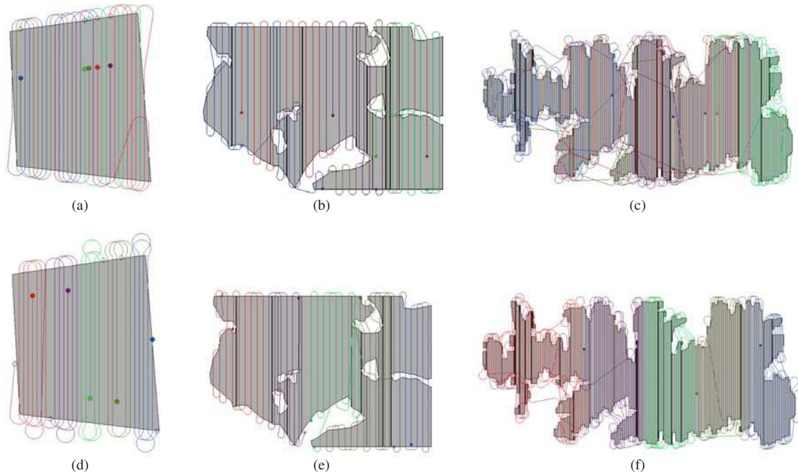
Fig. 3. A simulation instance of DCRC (first row) and DCAC (second row) algorithms with 5 robots performing coverage over the area of interest indicated in gray, where the first column shows a small segment in the Lake Murray ( 200 \text{ m} \times 200 \text{ m} ); second column, Rural Quebec ( 13 \text{ km} \times 10 \text{ km} ); third column, the complete Lake Murray ( 25 \text{ km} \times 25 \text{ km} ).
