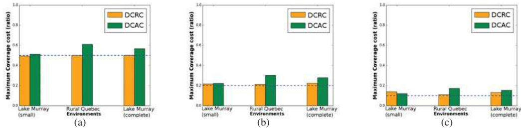
Fig. 4. The comparison of actual maximum coverage cost and the ideal cost for three different environments for (a) k = 2 (b) k = 5 and (c) k = 10 robots.
