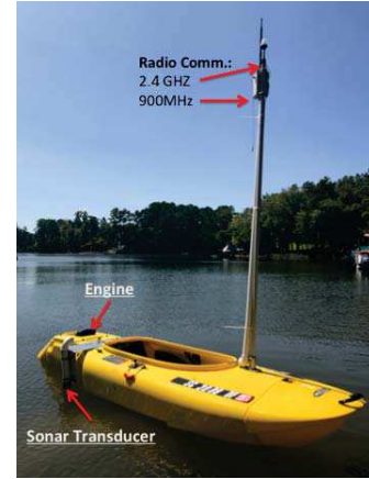
Fig. 2. Experimental ASV Setup.
