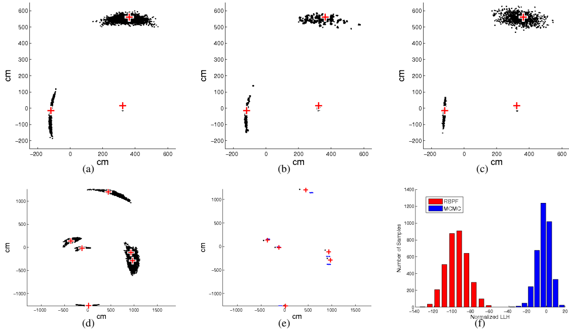
Fig. 3. Results for 4 step paths through a 3 sensor network for the algorithms: (a) MCMC (b) RBPF ( K = 5000 ), and (c) EKF. Data obtained for 50 step paths through a 6 sensor network for the algorithms: (d) MCMC (e) RBPF ( K = 20000 ), (black particles) and EKF (blue uncertainty ellipses). For all of (a-e), crosses indicate the ground truth sensor positions. (f) Histogram comparing the relative log likelihoods (LLH) of the final configuration samples obtained from the MCMC and RBPF ( k = 20000 ) techniques for the simulation result shown in (d). The likelihoods were normalized such that ground truth had a log likelihood of zero.
