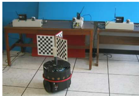
Fig. 1. The components of the camera sensor network used in the experimental results of the paper.
