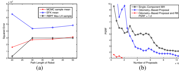
Fig. 4. (a) Squared error of MLE of sensor positions as a function of robot path length through a 6 sensor network; (the same simulation presented in Figure 3(d)). The RBPF sample mean result was slightly poorer than the RBPF maximum likelihood sample, so it is not presented. (b) Potential scale reduction factor (PSRF) as a function of computational effort for 4 sensor, 12 path length scenario, with 4 restarts.
