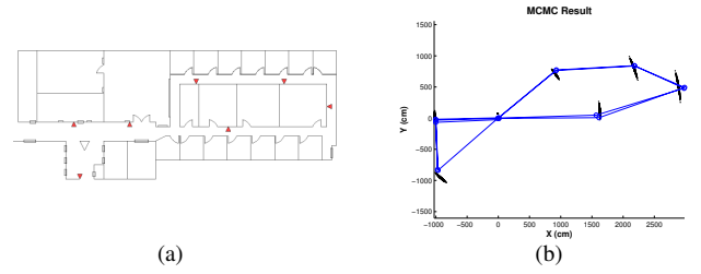
Fig. 5. (a) Approximate floor plan showing camera locations during the experiment. (b) A graphical representation of inferred positions. Lines summarize a section of the robot's actual path (hidden for clarity) by the relative poses between camera positions.
