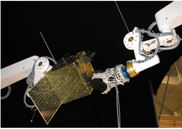
Fig. 7. The SARAH hand grasping the target satellite.
