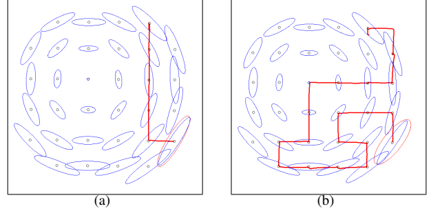
Figure 2. Effect of \alpha on the resulting solution path starting from the same source node to target node. (a) \alpha = 1.0 , which is equivalent to Dijkstra's shortest path (b) \alpha = 0.0 , heuristic search considering only map uncertainty reduction.
