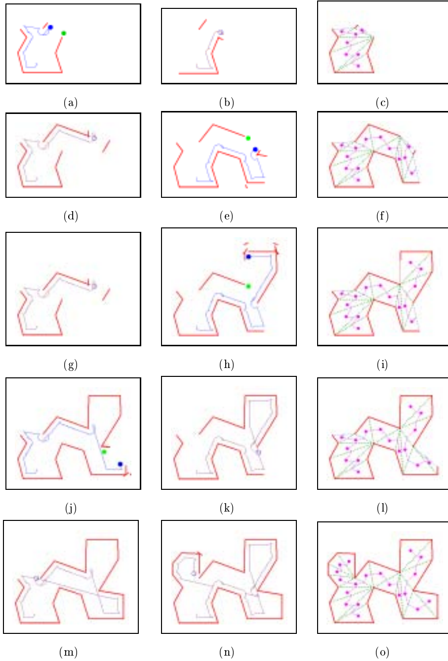
Figure 11. Exploring an unknown environment with two occluding vertices: The first column illustrates the trajectory of Robot 0 . (a,d,g,j,m). The second column illustrates the trajectory of Robot 1 (b,e,h,k,n). Finally the third column presents the map up to that point (c,f,i,l,o). (See text Section 7.1.1).
