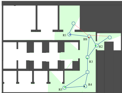
Fig. 1. Representation of the constrained exploration problem, where robots (R1-R5) need to be connected, either directly or in multihop, to the base station (BS). The explored area (green) together with the communication graph built by considering a conservative range line-of-sight communication model (blue) are illustrated. The red dashed lines indicate links that can be added with the approach proposed in this paper.
