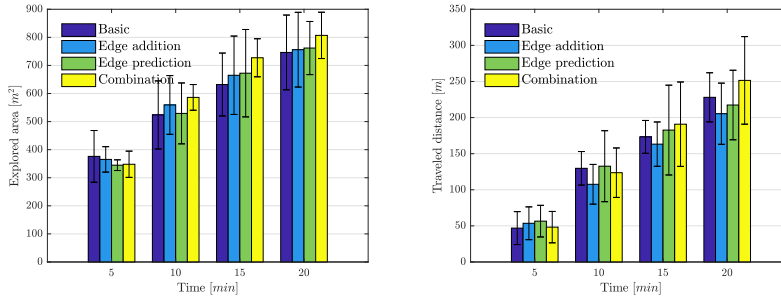
Fig. 5. Performance in Cluttered.
