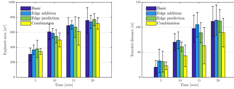
Fig. 4. Performance in Open.
