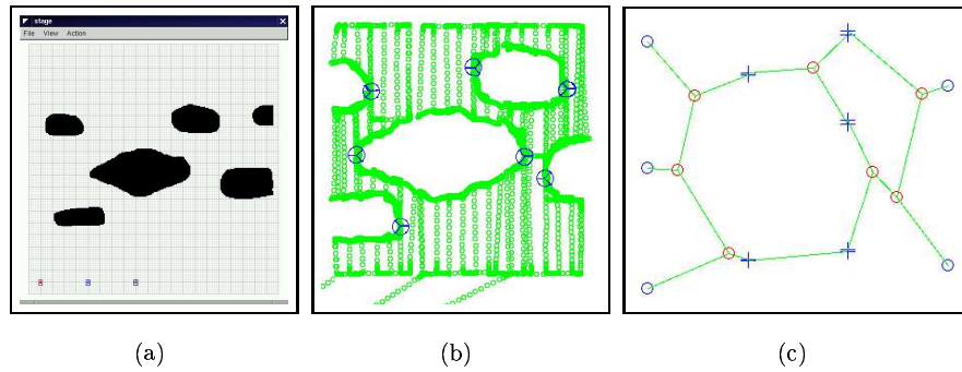
Figure 5. (a) The environment and the three robots at the starting position in Stage. (b) The traces of the robots (marked as circles which are smaller than the footprint) and the critical points encountered. (c) The augmented Reeb graph with the critical points (circles) and the Steiner points (crosses).
