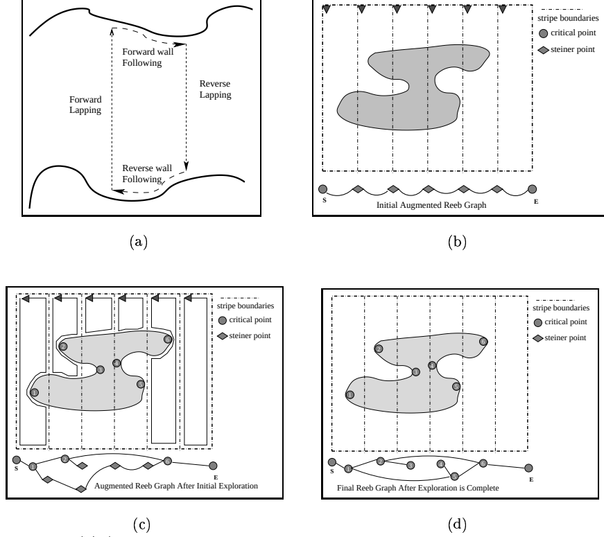
Figure 4. (a) A simple cycle path consisting of forward lapping, forward wall following, reverse lapping and reverse wall following. (b) Simple environment with initial Augmented Reeb Graph. (c) Initial exploration of stripes. (d) The final Reeb Graph after exploration is complete.
